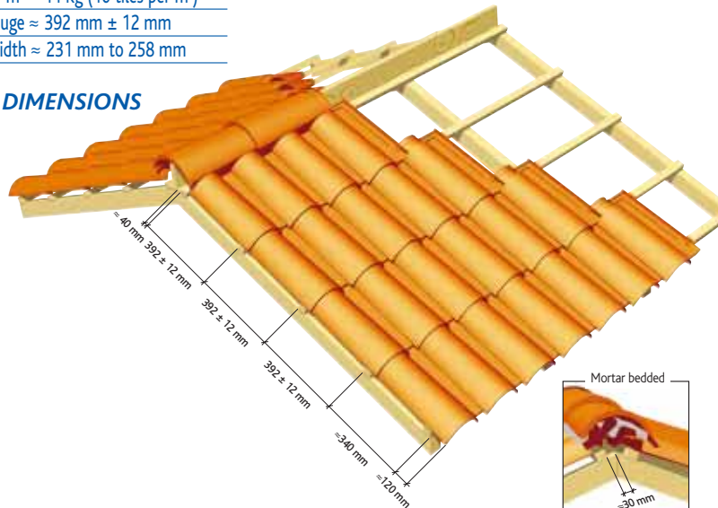
Installation without round verge tiles
