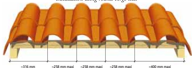
Installation using round verge tiles
