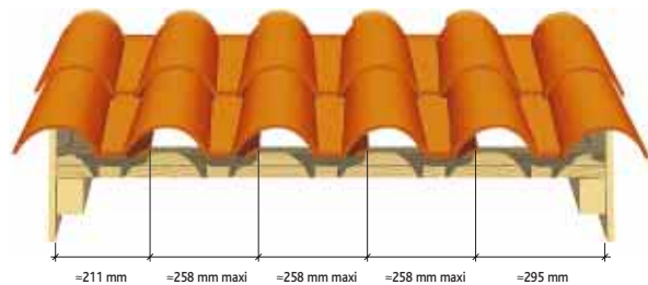
Installation using round verge tiles
